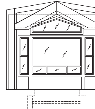
Catalina Alternate 3000 Series Front Elevation
